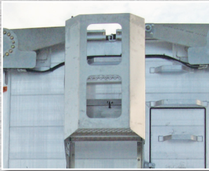
Front Catwalk
